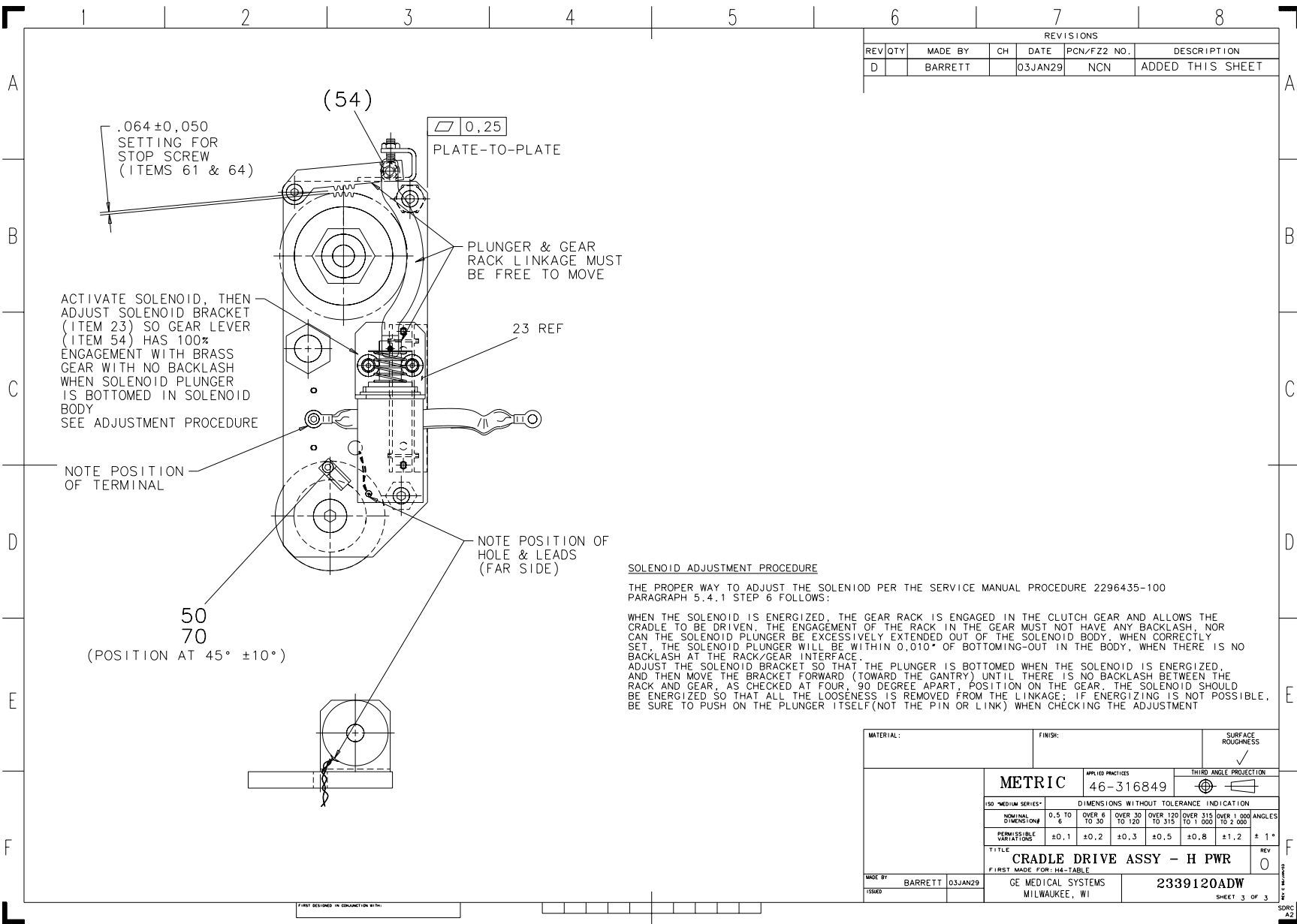
Figure 2-14 Cradle Drive Assembly (2339120, sheet 3, rev 0)
